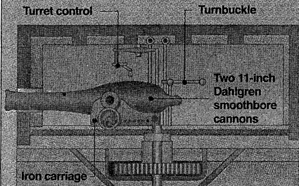
Cross-section of turret
